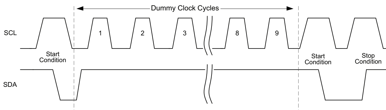
Figure 6-4. Software Reset
