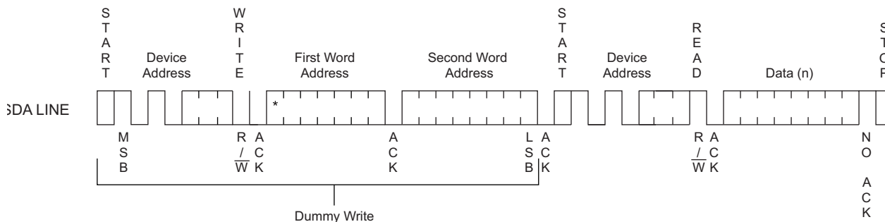
Figure 9-2. Random Read
