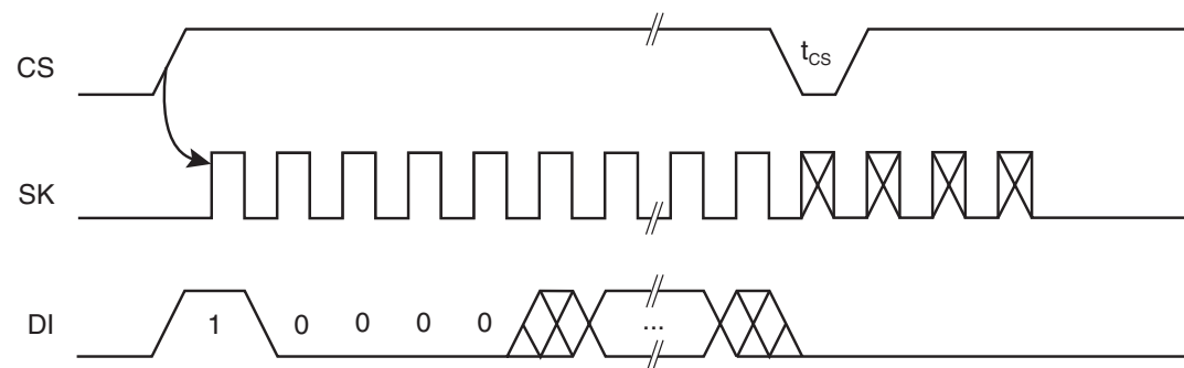
Figure 5. EWDS Timing
