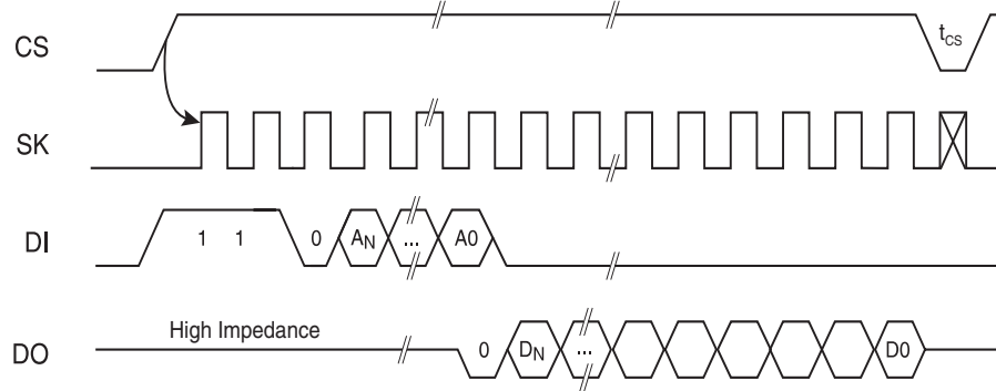
Figure 3. READ Timing
