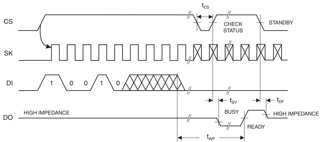
Figure 9. ERAL Timing (1)
