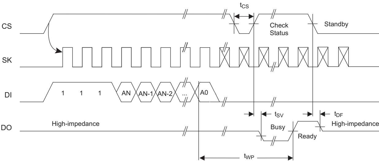
Figure 6-2. ERASE Timing
