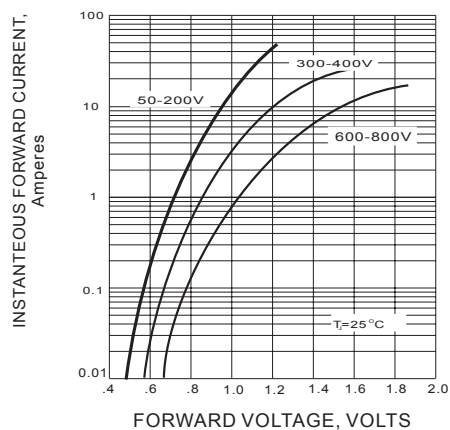
Fig.2 FORWARD CHARACTERISTICS
