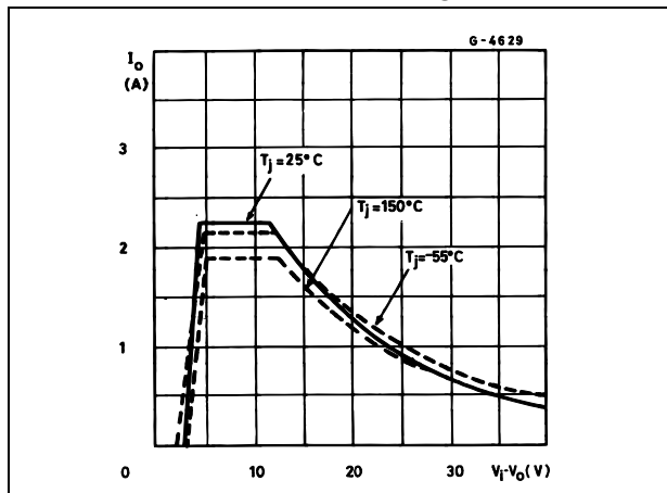
Figure 3. Output current vs. input-output differential voltage
