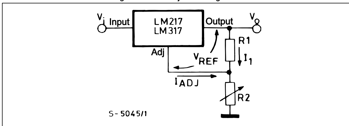
Figure 6. Basic adjustable regulator
