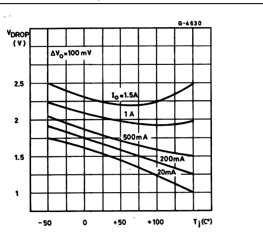
Figure 4. Dropout voltage vs. junction temperature
