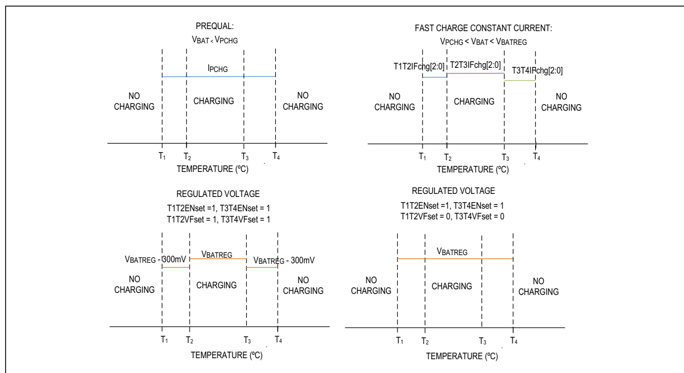
Figure 6. Thermistor Monitoring
