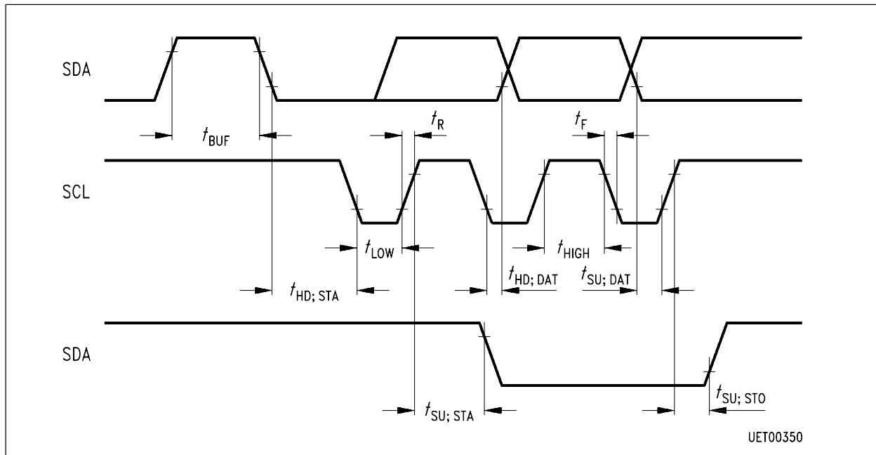
Figure 2 Timing Conditions for the I²C Bus
