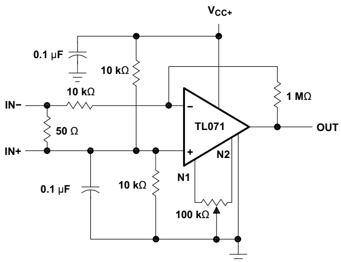
Figure 28. AC Amplifier
