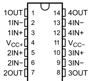
TL074x D, J, N, NS, PW, and W Package 14-Pin SOIC, CDIP, PDIP, SO and CFP Top View
